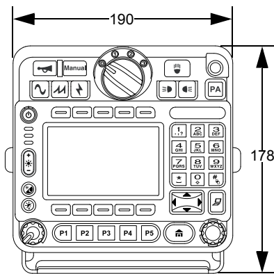
Figure 1-21. Front View of O9 Control Head with Trunnion
