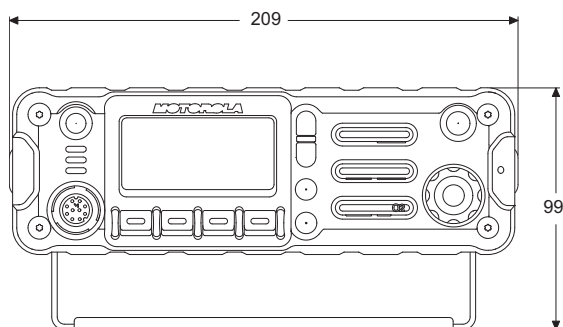
Figure 1-15. Front View of O2 Control Head with Remote Mount and Trunion
