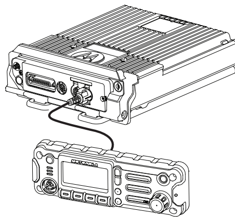
Figure 1-34. Remote Mount Configuration with High Power (100W) Radio Transceiver and O2 Control Head
