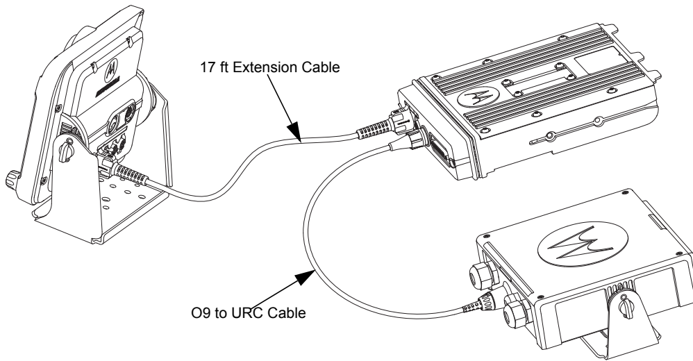
Figure 1-40. Remote Mount Configuration with Mid Power Radio Transceiver, Universal Relay Controller and O9 Control Head (URC is optional)
