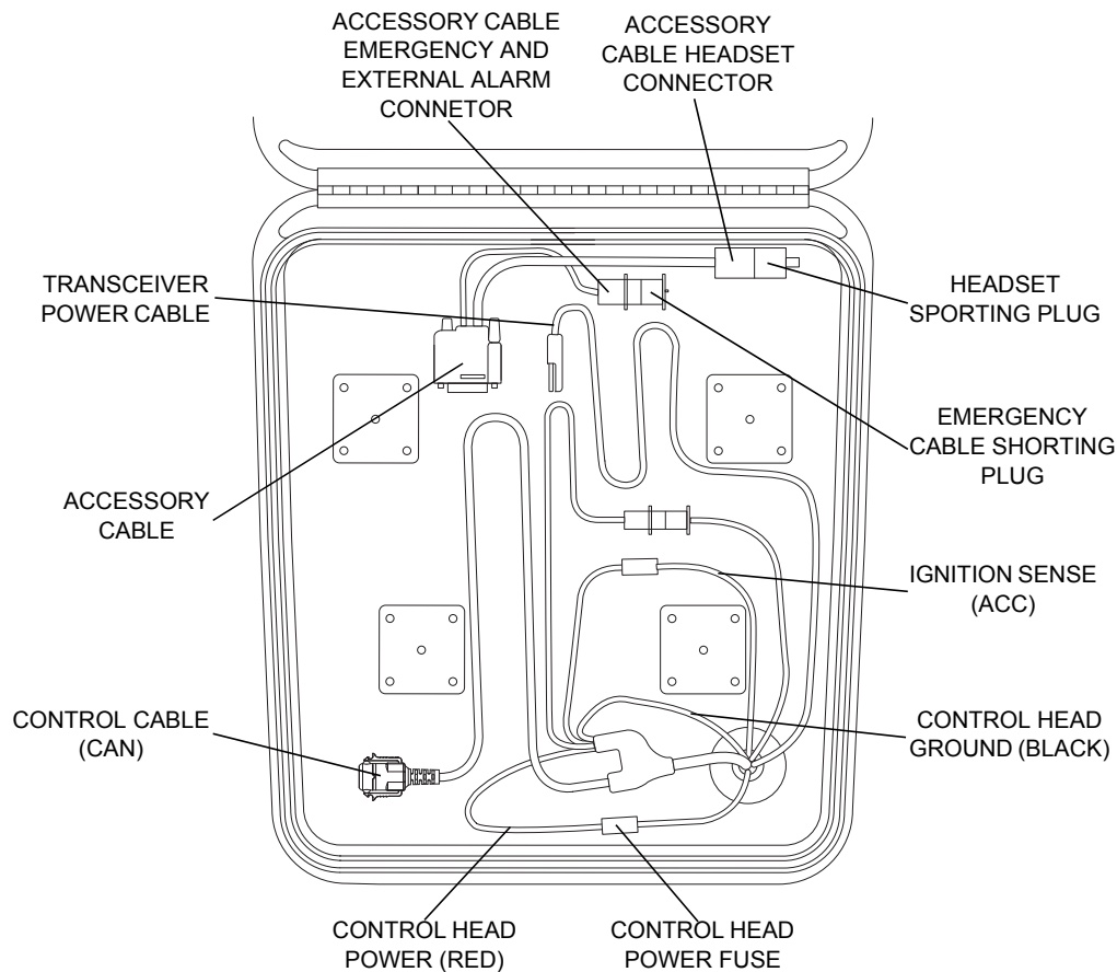
Figure 5-16. Installing Cables
