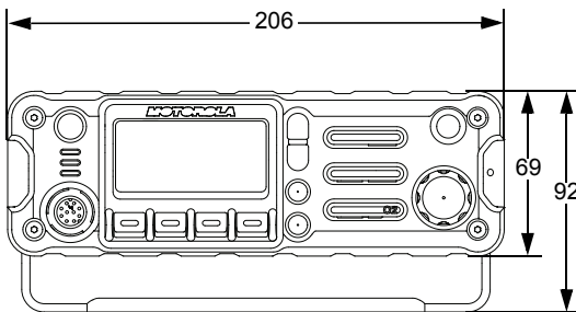
Figure 1-9. Front View of O2 Control Head Attached to APX 7500 Mid Power Dash Mount Transceiver and Trunion
