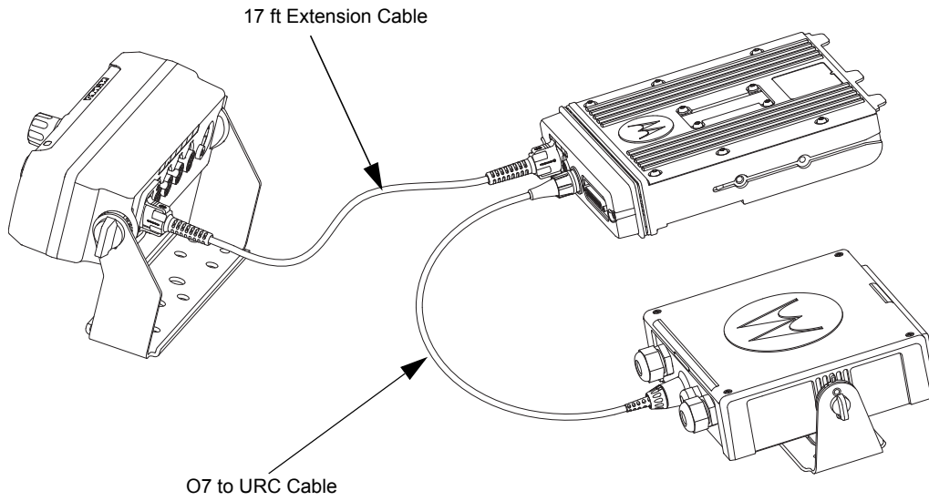
Figure 1-39. Remote Mount Configuration with Mid Power Radio Transceiver, Universal Relay Controller and O7 Control Head (URC is optional)
