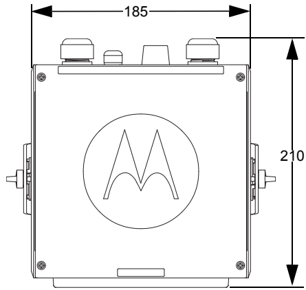
Figure 1-23. Top View of O9 Universal Relay Controller with Trunnion (URC is an orderable accessory)
