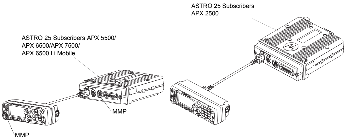
Figure 1-31. Remote Mount Configuration with Mid Power Transceiver, Transceiver Interface Board, CHIB Rear Assembly and O5 Control Head
