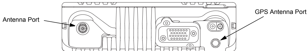
Figure 5-10. APX 2500/APX 4500/APX 1500 Antenna Band Identification
