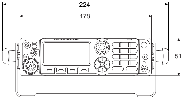
Figure 1-11. Front View of O7 Control Head Attached to APX 2500 Mid Power Dash Mount Transceiver and Trunion
