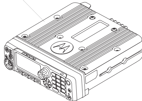
Figure 1-28. Dash Mount Configuration for O7 Control Head
