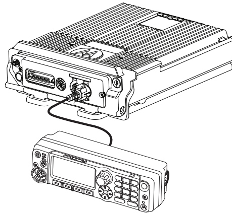
Figure 1-37. Remote Mount Configuration with High Power (100W) Radio Transceiver and O7 Control Head
