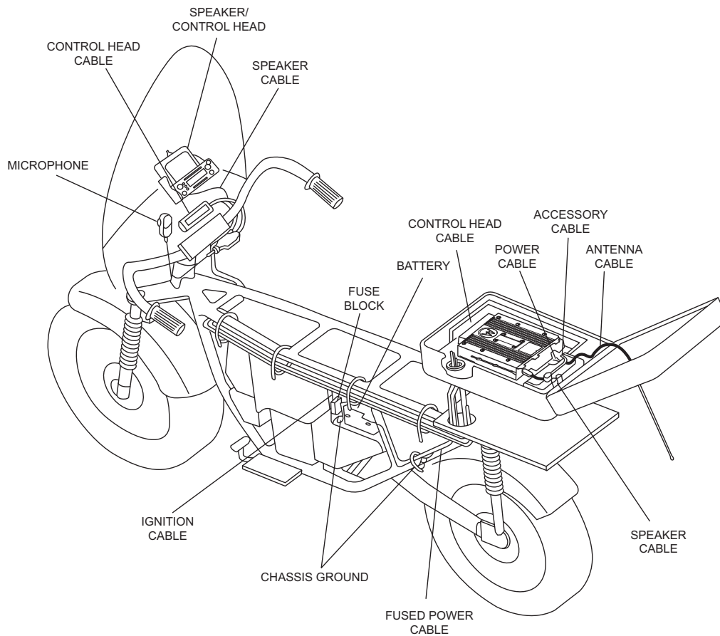
Figure 5-14. Cable Routing
