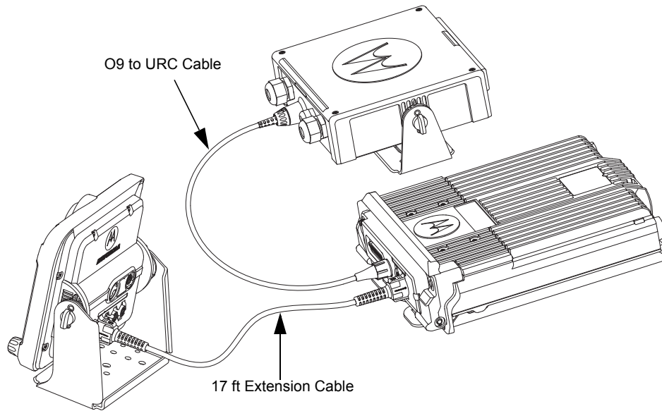
Figure 1-42. Remote Mount Configuration with High Power (100W) Radio Transceiver, Universal Relay Controller and O9 Control Head (URC is optional)
