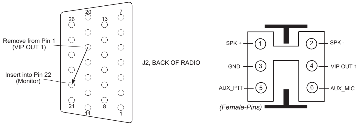
Figure 5-18. Motorcycle Wiring Harness Rework
