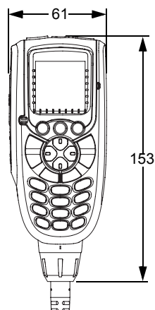
Figure 1-13. Front View of O3 Control Head with Coiled Cable
