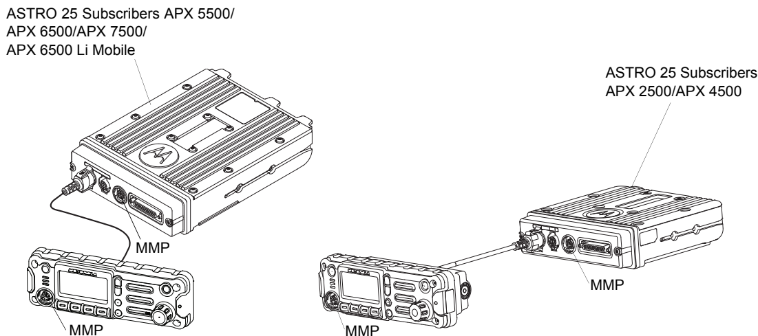
Figure 1-29. Remote Mount Configuration with Mid Power Transceiver, Transceiver Interface Board, CHIB Rear Assembly and O2 Control Head
