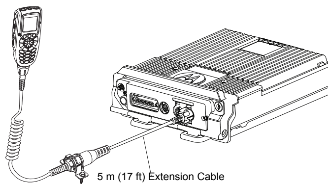
Figure 1-35. Remote Mount Configuration with High Power (100W) Radio Transceiver and O3 Control Head
