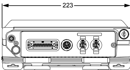
Figure 1-7. Front View of APX 7500 High Power (100W) Transceiver and Trunion
