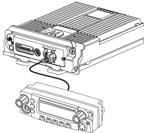
Figure 1-36. Remote Mount Configuration with High Power (100W) Radio Transceiver and O5 Control Head
