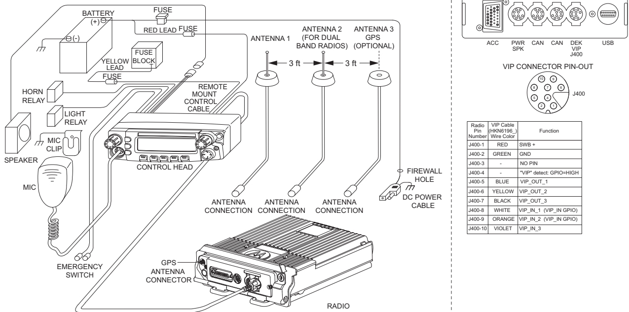
Figure 2-14. Radio Installation (O5 High Power Remote Mount)
