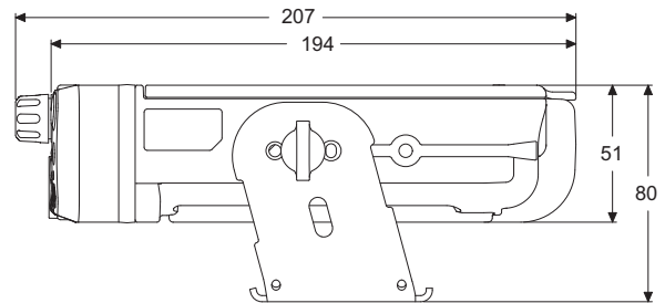
Figure 1-12. Side View of O7 Control Head Attached to APX 2500 Mid Power Dash Mount Transceiver and Trunion
