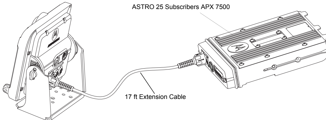
Figure 1-33. Remote Mount Configuration with Mid Power Transceiver, Transceiver Interface Board and O9 Control Head
