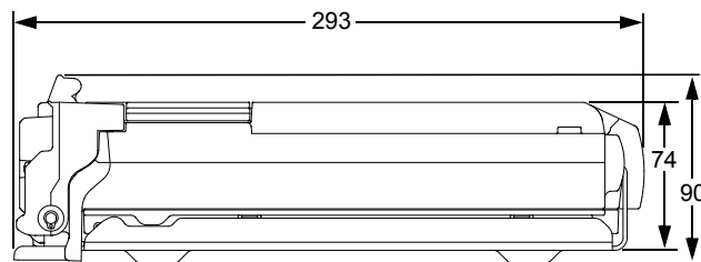
Figure 1-8. Side View of APX 7500 High Power (100W) Transceiver and Trunion
