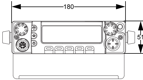
Figure 1-17. Front View of O5 Control Head with Remote Mount and Trunnion
