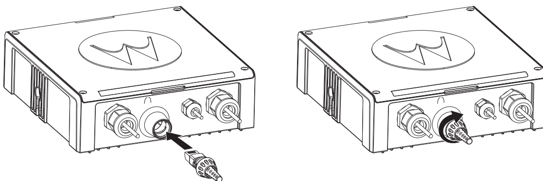
Figure 3-7. O7/O9 to URC Cable Installation
