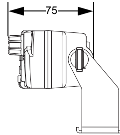
Figure 1-18. Side View of O5 Control Head with Remote Mount and Trunnion
