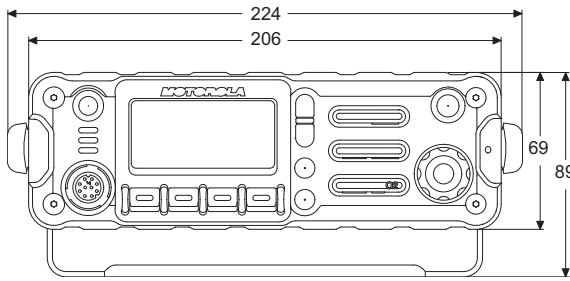
Figure 1-5. Front View of APX 2500/APX 4500/APX 1500 Mid Power Dash Mount Transceiver and Trunion
