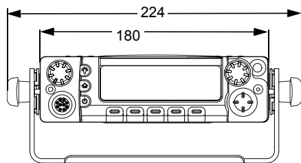
Figure 1-3. Front View of O5 Control Head Attached to APX 2500/4500 Mid Power Dash Mount Transceiver and Trunnion
