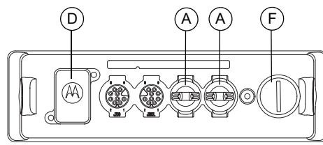
Control Head (Rear)
