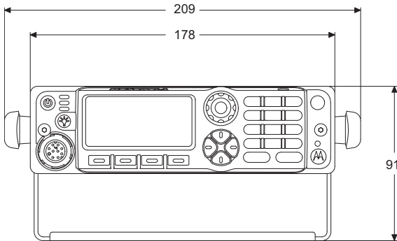
Figure 1-19. Front View of O7 Control Head with Remote Mount and Trunnion
