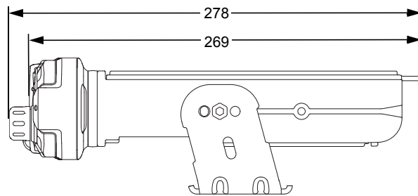
Figure 1-10. Side View of O2 Control Head Attached to APX 7500 Mid Power Dash Mount Transceiver and Trunion
