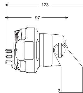
Figure 1-16. Side View of O2 Control Head with Remote Mount and Trunion
