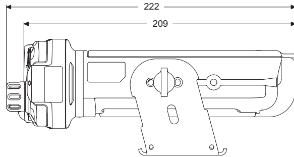
Figure 1-6. Side View of APX 2500/APX 4500/APX 1500 Mid Power Dash Mount Transceiver and Trunion
