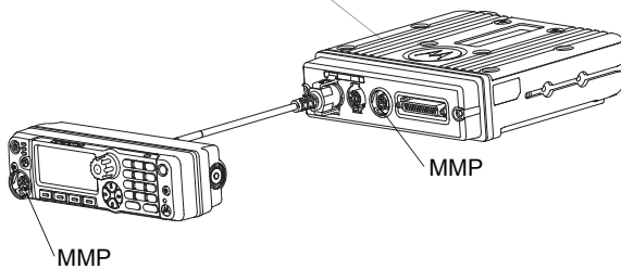
Figure 1-32. Remote Mount Configuration with Mid Power Transceiver, Transceiver Interface Board, CHIB Rear Assembly and O7 Control Head
