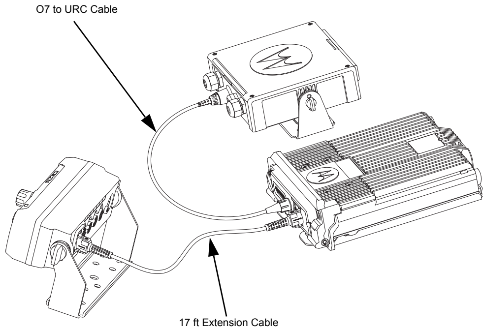
Figure 1-41. Remote Mount Configuration with High Power (100W) Radio Transceiver, Universal Relay Controller and O7 Control Head (URC is optional)
