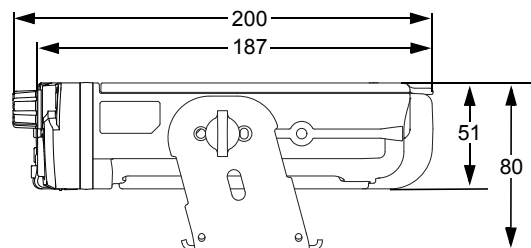
Figure 1-4. Side View of O5 Control Head Attached to APX 2500/4500 Mid Power Dash Mount Transceiver and Trunnion
