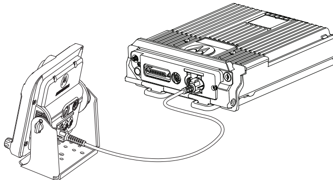
Figure 1-38. Remote Mount Configuration with High Power (100W) Radio Transceiver and O9 Control Head
