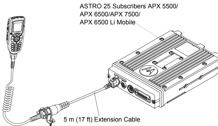
Figure 1-30. Remote Mount Configuration with Mid Power Transceiver, Transceiver Interface Board and O3 Control Head
