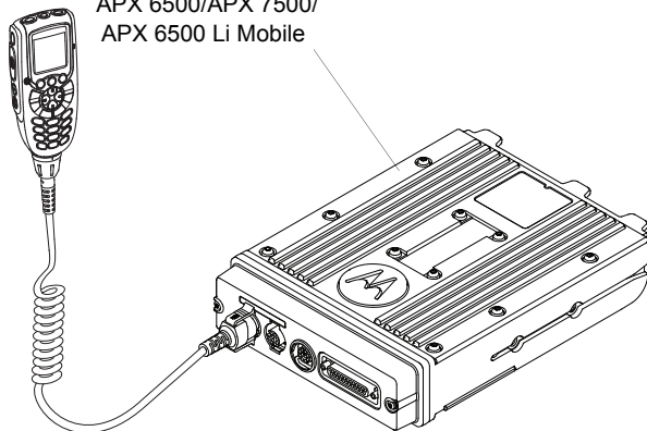
Figure 1-26. Dash Mount Configuration for O3 Control Head
