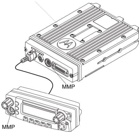
Figure 1-31. Remote Mount Configuration with Mid Power Transceiver, Transceiver Interface Board, CHIB Rear Assembly and O5 Control Head
