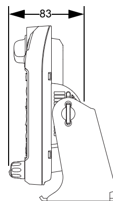
Figure 1-22. Side View of O9 Control Head with Trunnion
